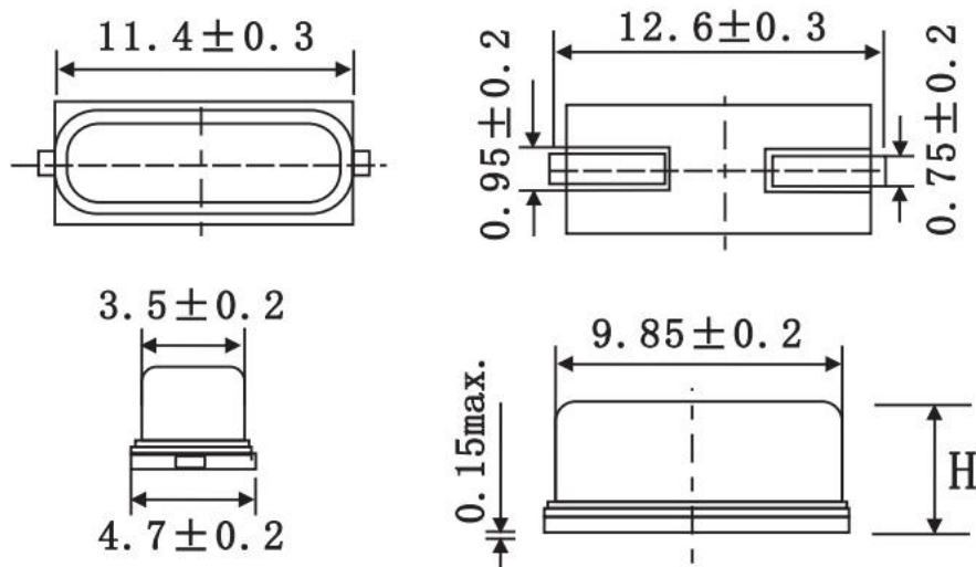
49S/SMD-2PIN
